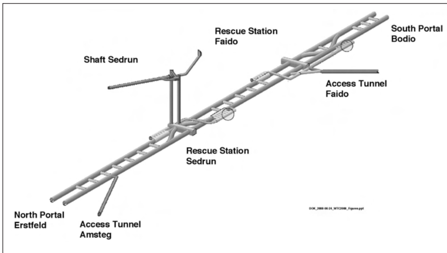
Figure 4 - Gotthard Base Tunnel
