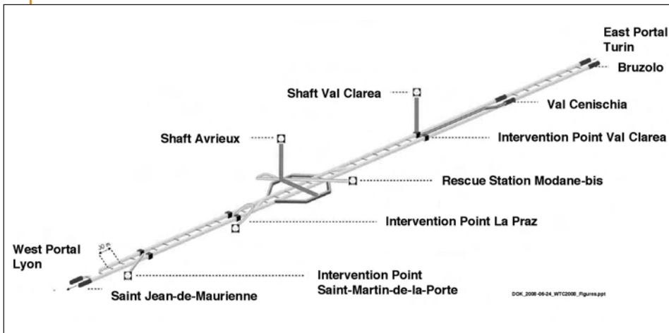
Figure 2 - Lyon-Turin Base Tunnel
